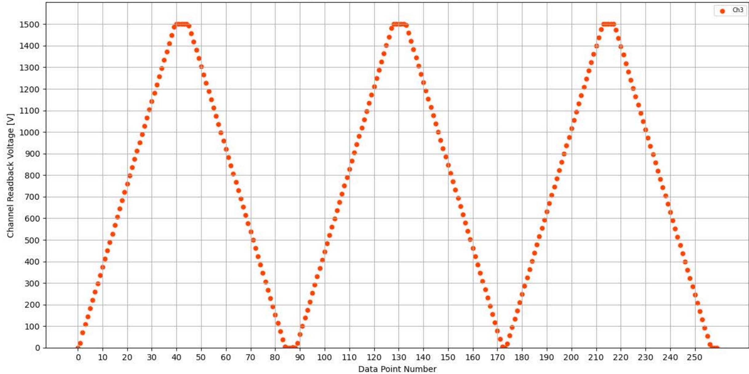
Voltage Ramp Test (Python) Bd #299, Slot #1, Ch #3
