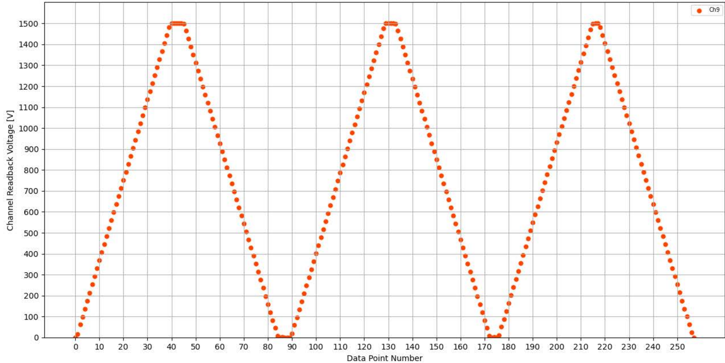
Voltage Ramp Test (Python) Bd #299, Slot #1, Ch #9
