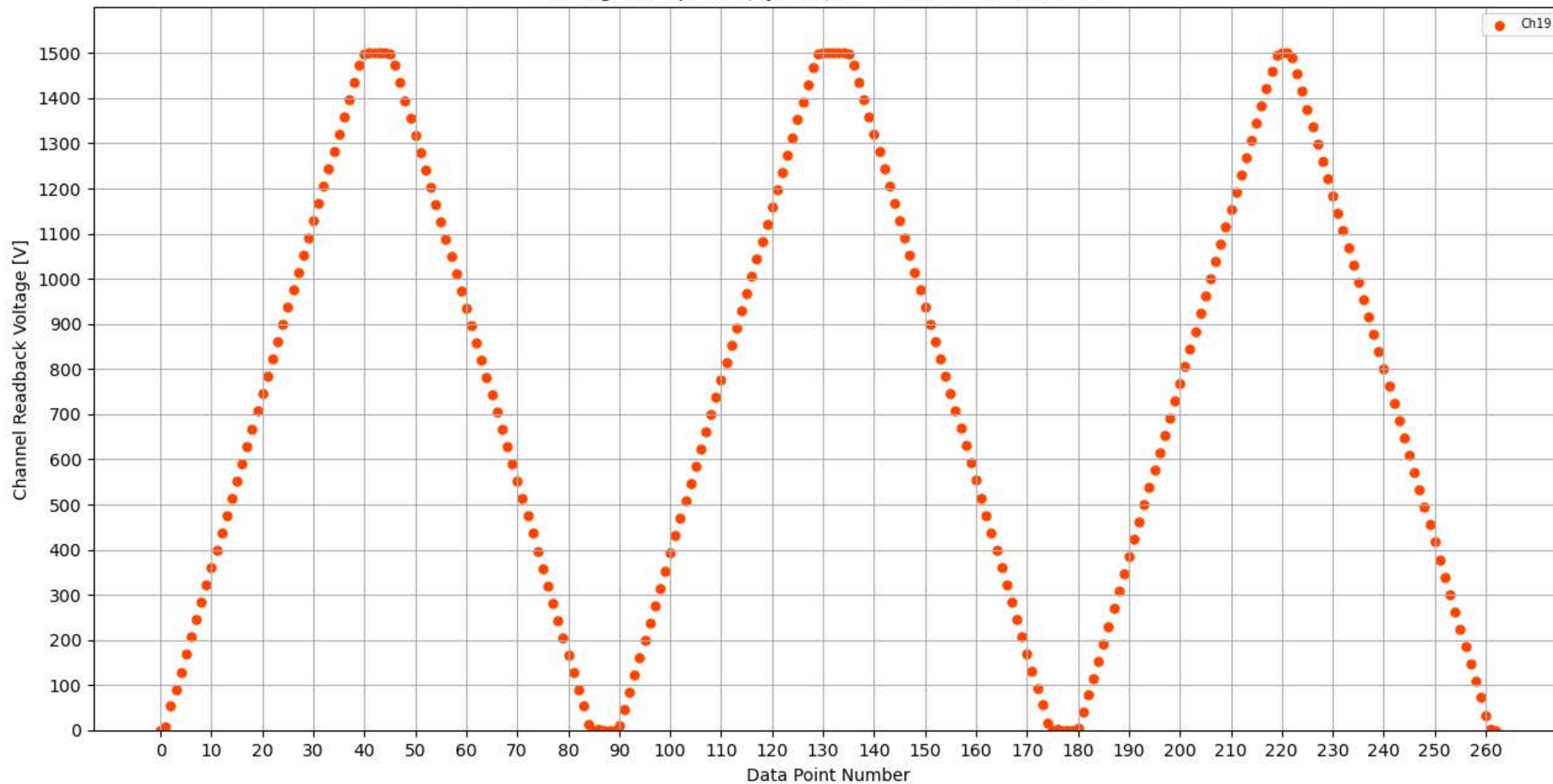
Voltage Ramp Test (Python) Bd #299, Slot #1, Ch #19
