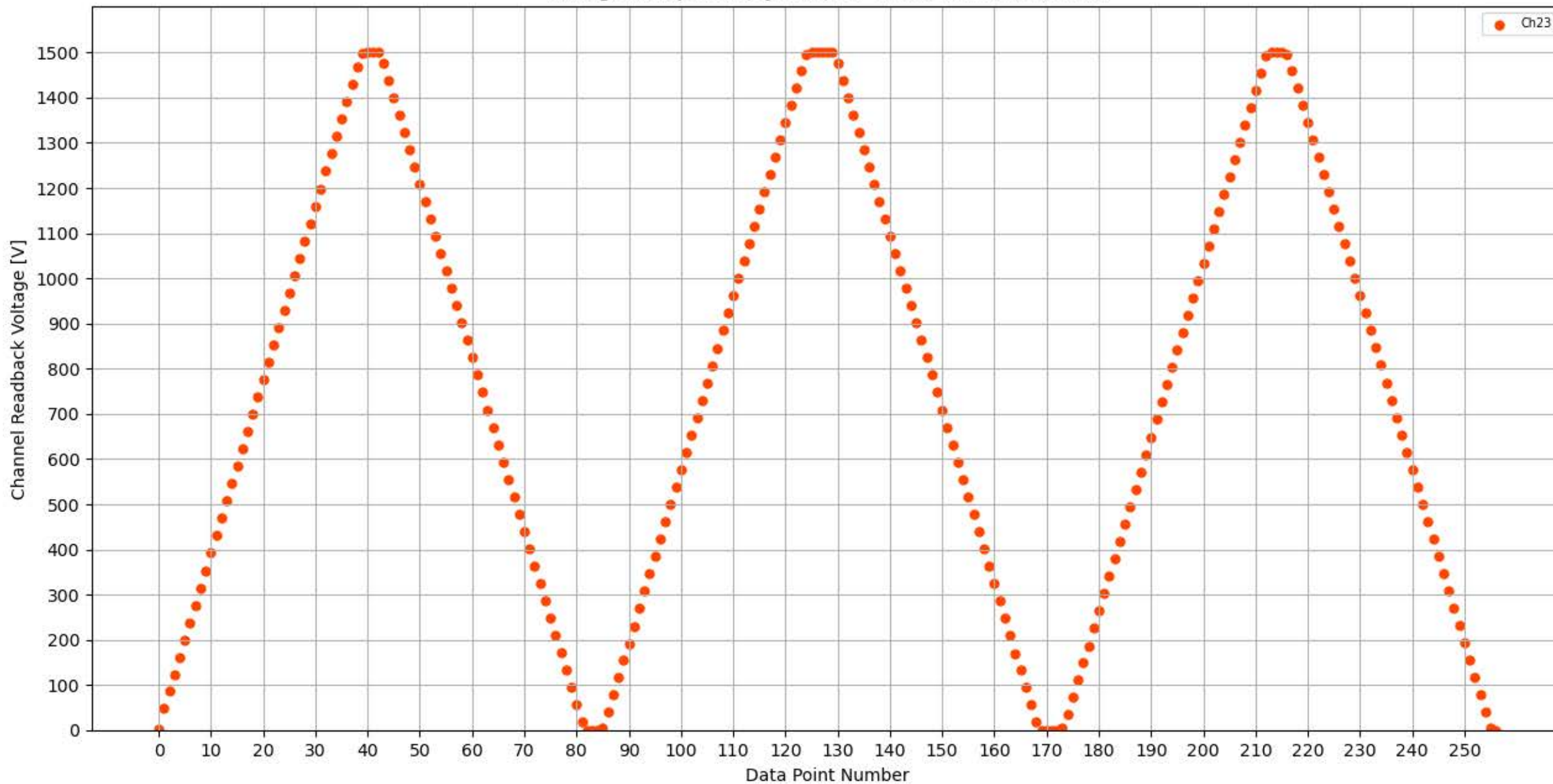
Voltage Ramp Test (Python) Bd #299, Slot #1, Ch #23
