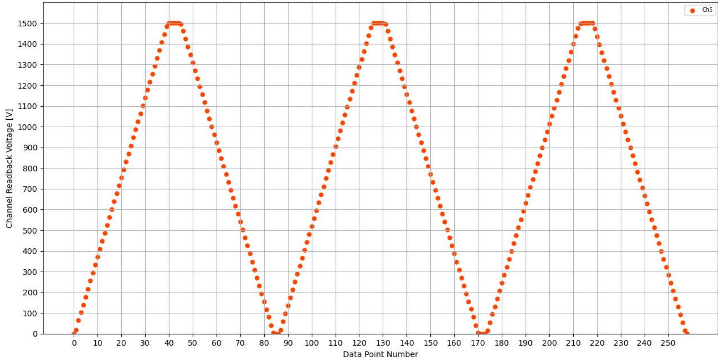
Voltage Ramp Test (Python) Bd #299, Slot #1, Ch #5
