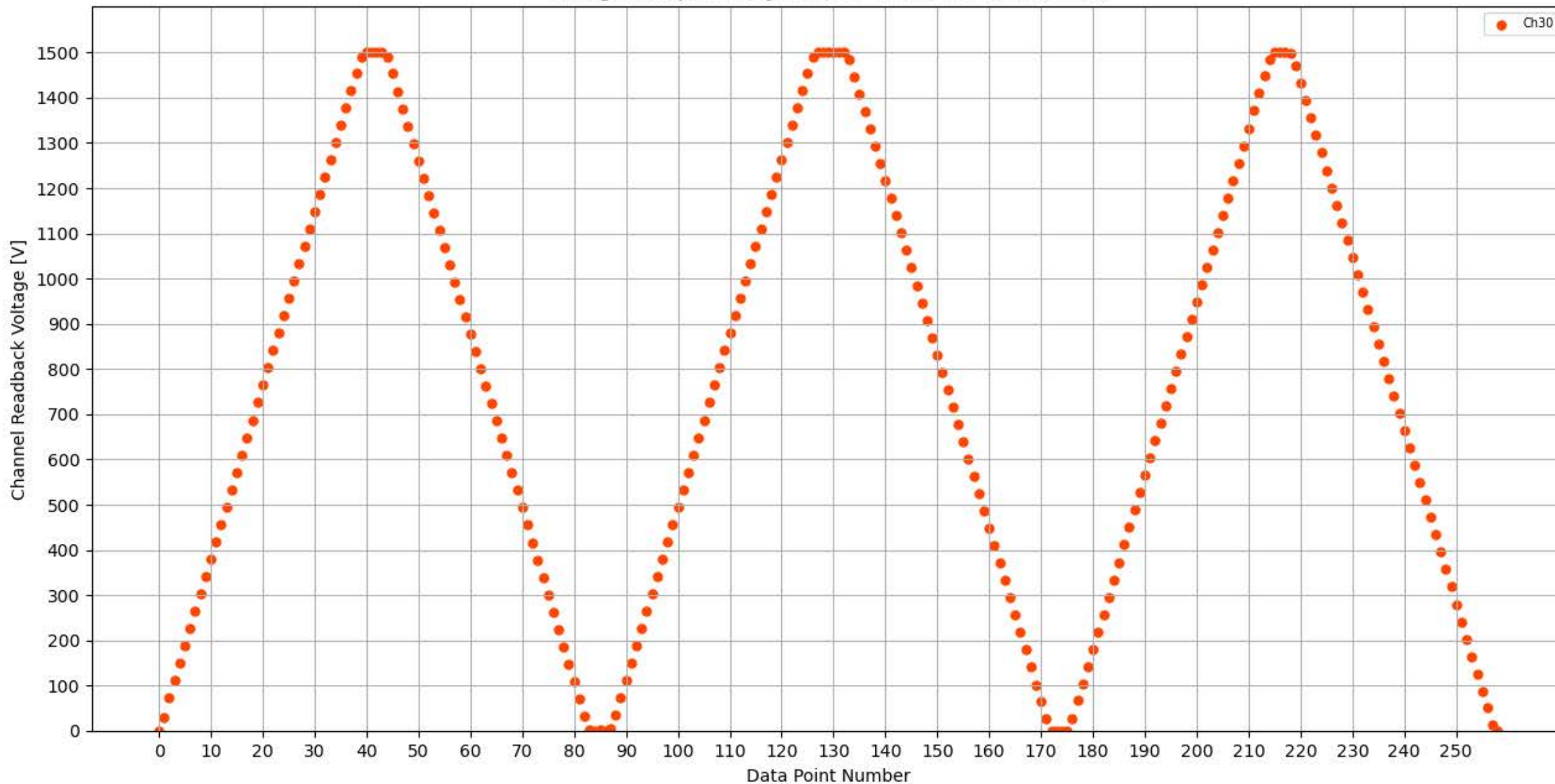
Voltage Ramp Test (Python) Bd #299, Slot #1, Ch #30
