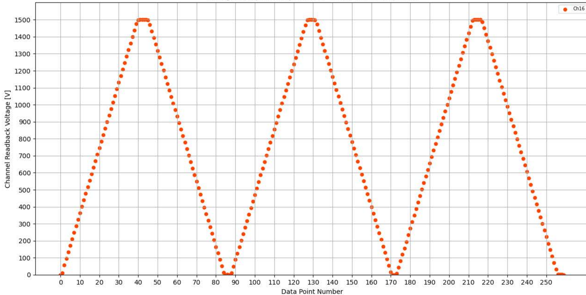
Voltage Ramp Test (Python) Bd #299, Slot #1, Ch #16
