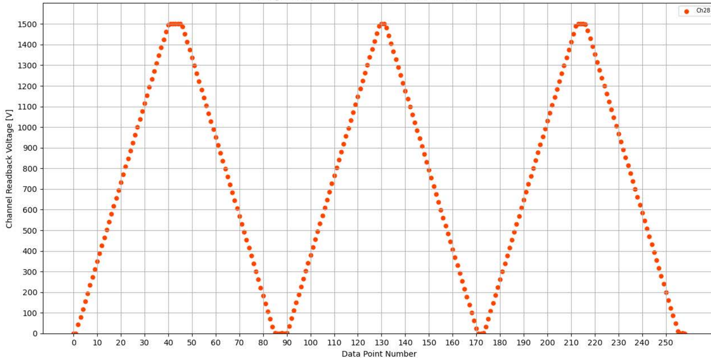
Voltage Ramp Test (Python) Bd #299, Slot #1, Ch #28
